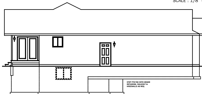
LEFT ELEVATION
